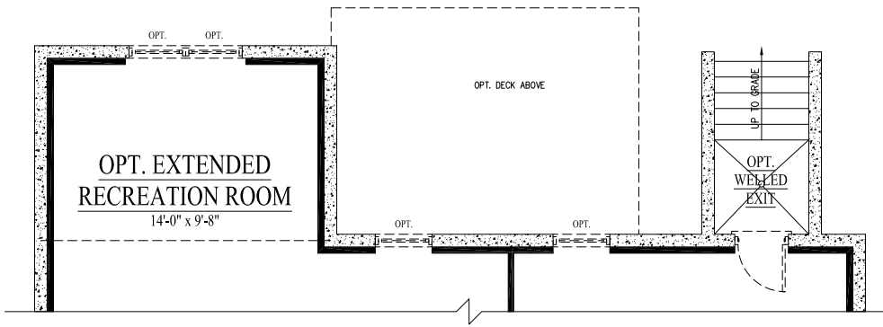
BASEMENT W/ OPT. SUNROOM
