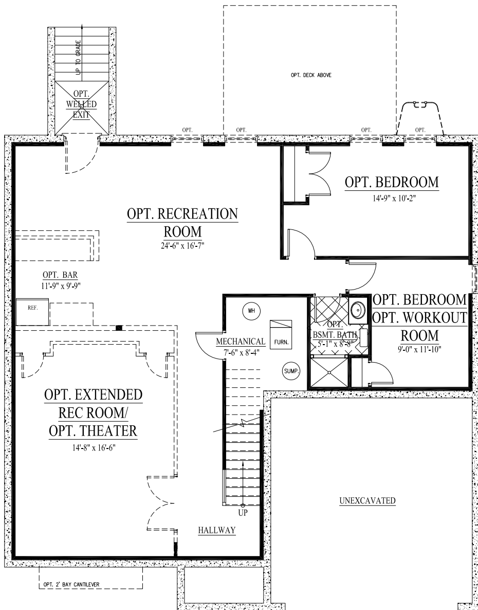
BASEMENT FLOORPLAN
