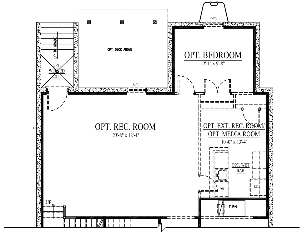
BASEMENT W/ SUNROOM OPTION
