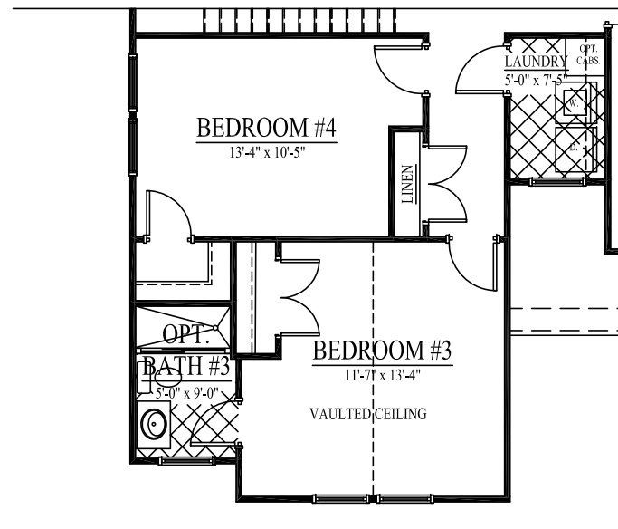
W/ VAULTED BEDROOM #3 (ELEVATION 2)
