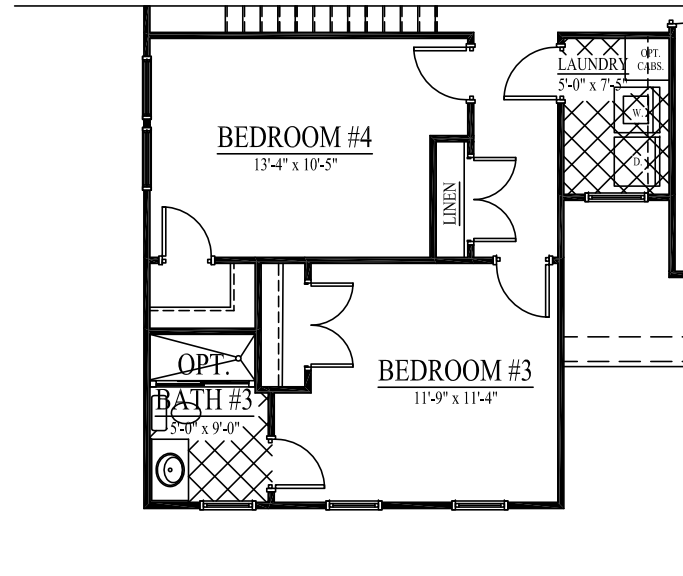
SECOND FLOOR W/ OPT. BATH #3
